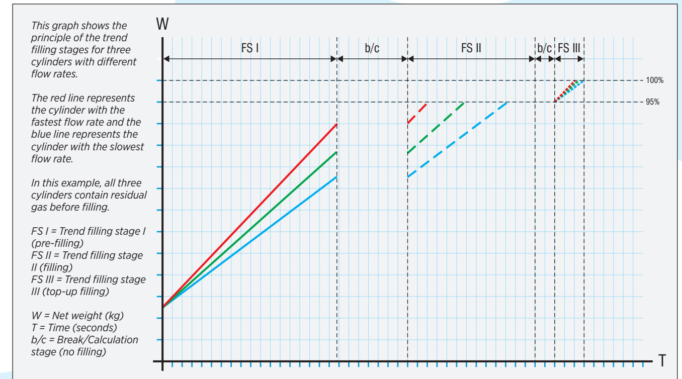
Trend filling stages for cylinders with residual gas
