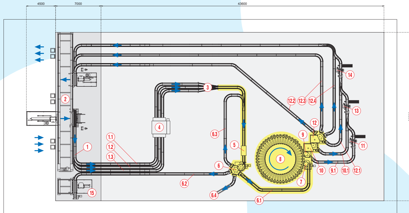
FLEXSPEED LAYOUT
